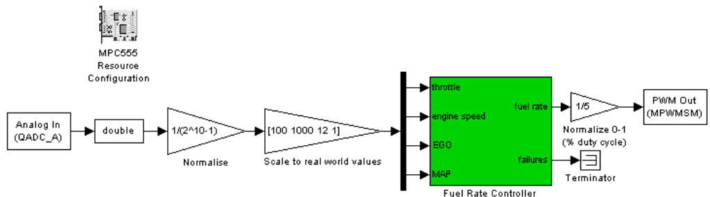
Fault-Tolerant Fuel Control System
